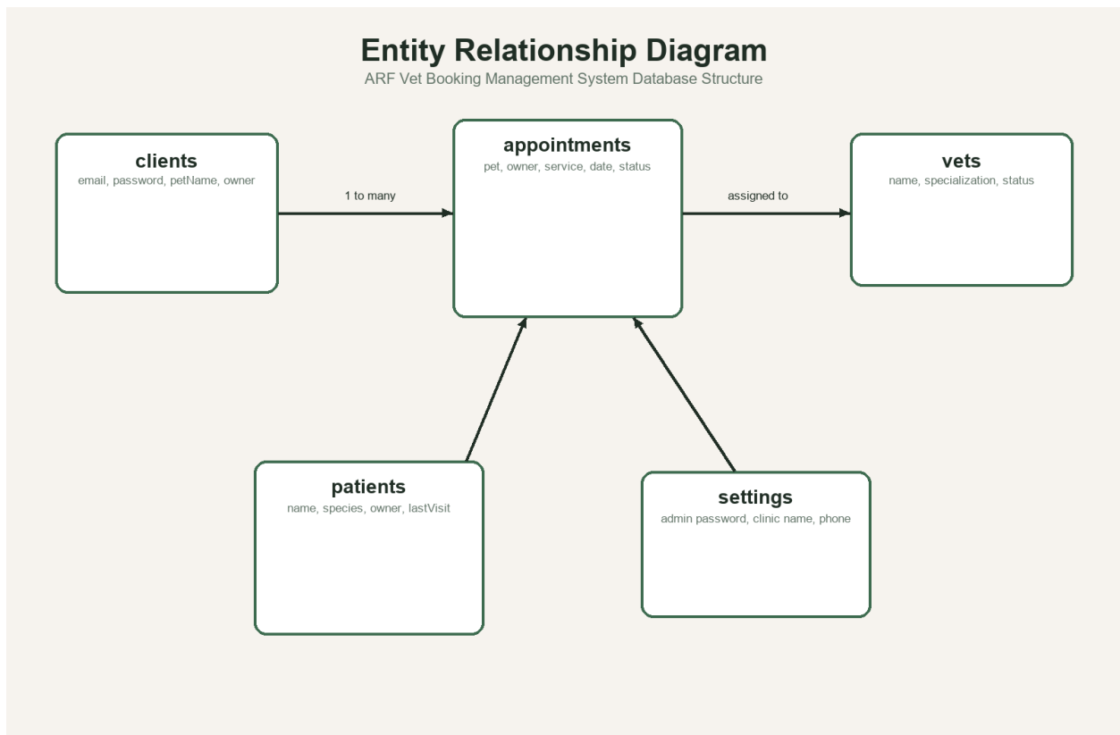
Figure 1. Entity Relationship Diagram of the ARF Portal
