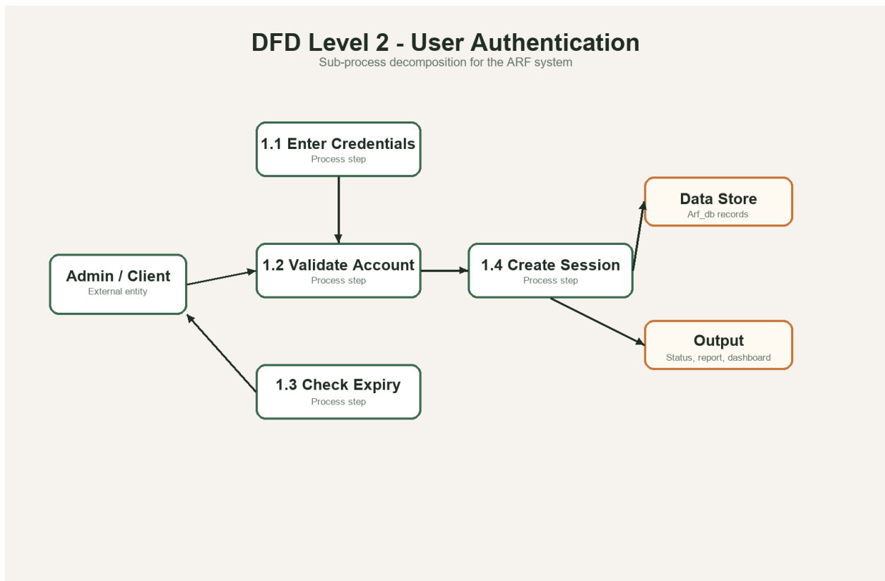
Figure 4. DFD Level 2 - Process 1.0: User Authentication
