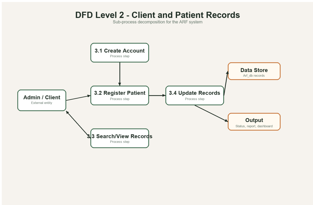
Figure 6. DFD Level 2 - Process 3.0: Client and Patient Records
