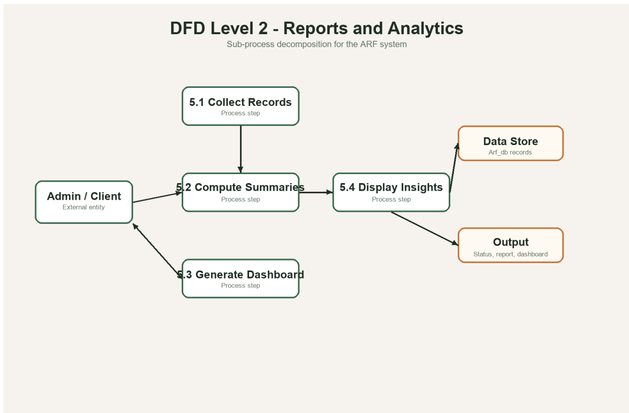
Figure 8. DFD Level 2 - Process 5.0: Reports and Analytics
