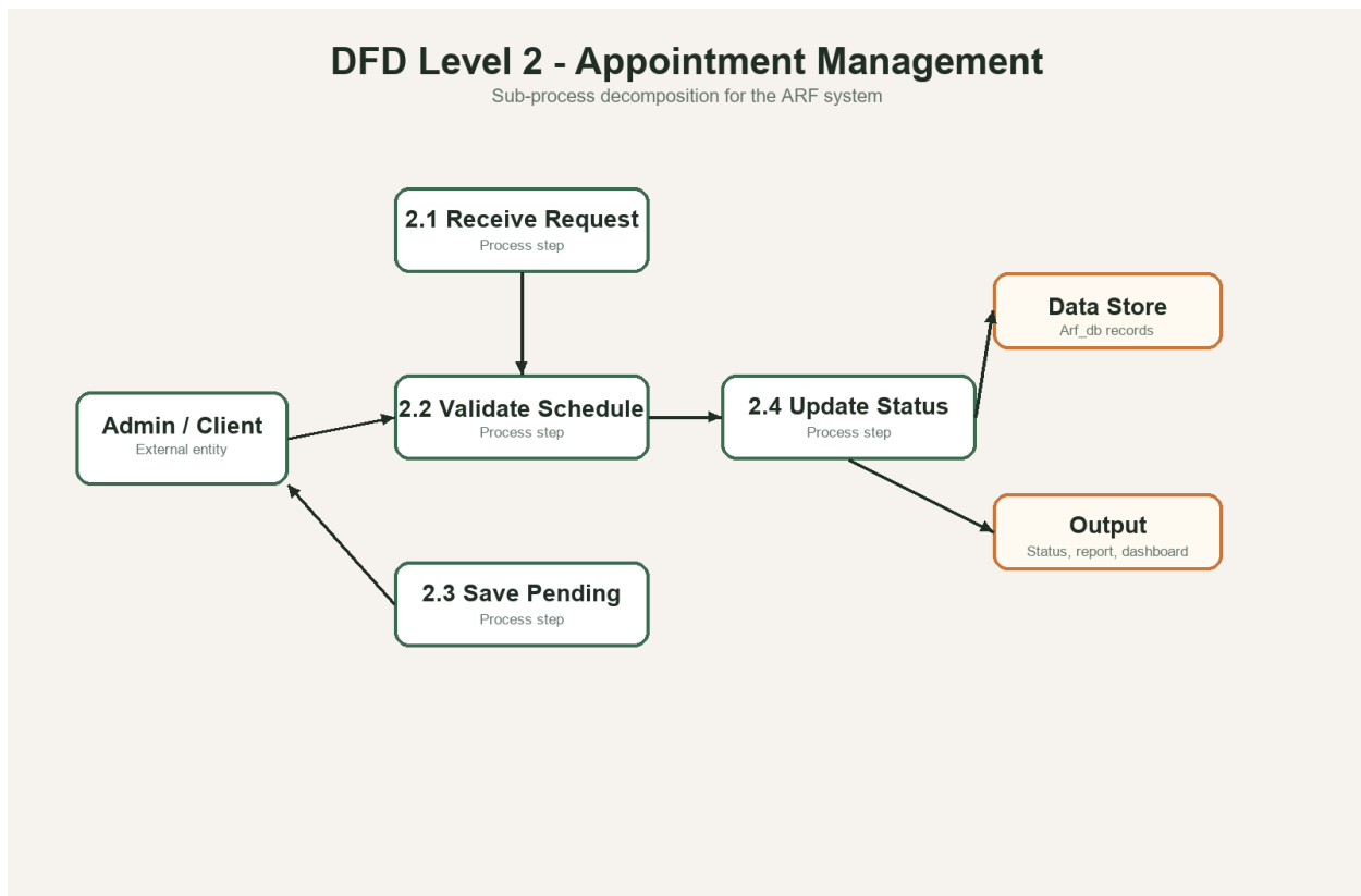
Figure 5. DFD Level 2 - Process 2.0: Appointment Management
