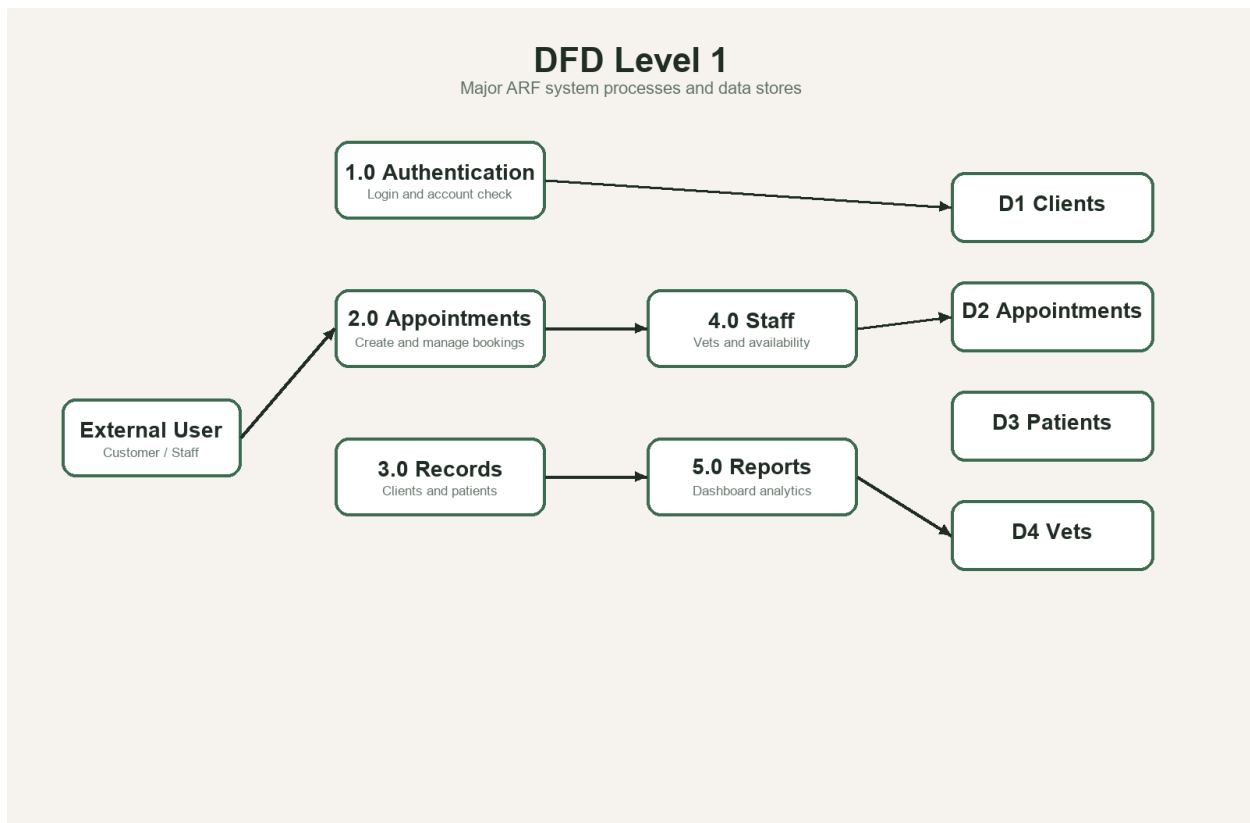
Figure 3. Data Flow Diagram (Level 1) of the ARF Portal
