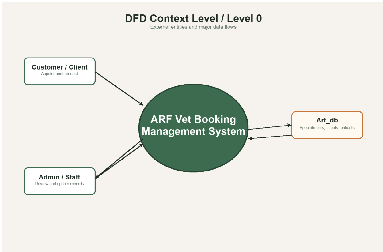
Figure 2. Context Diagram (Level 0) of the ARF Portal
