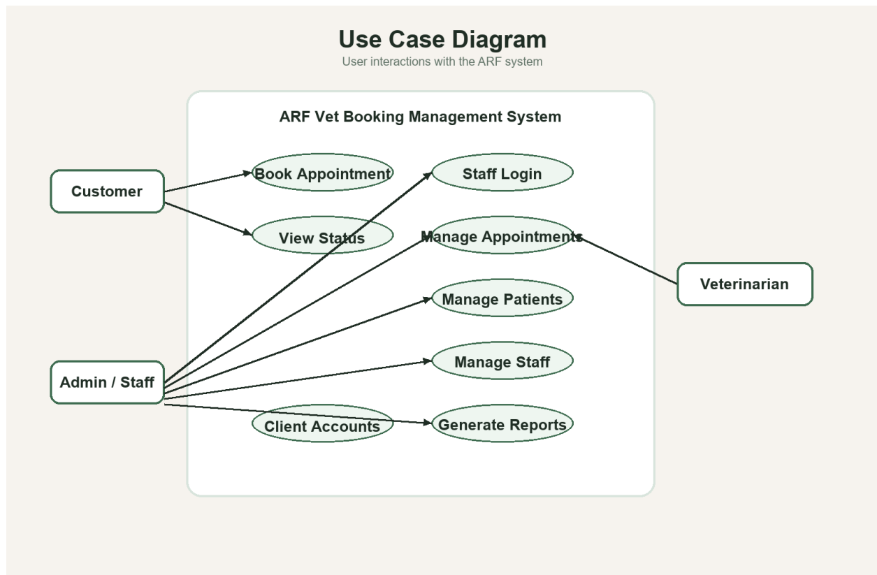
Figure 11. Use Case Diagram of the ARF Portal
