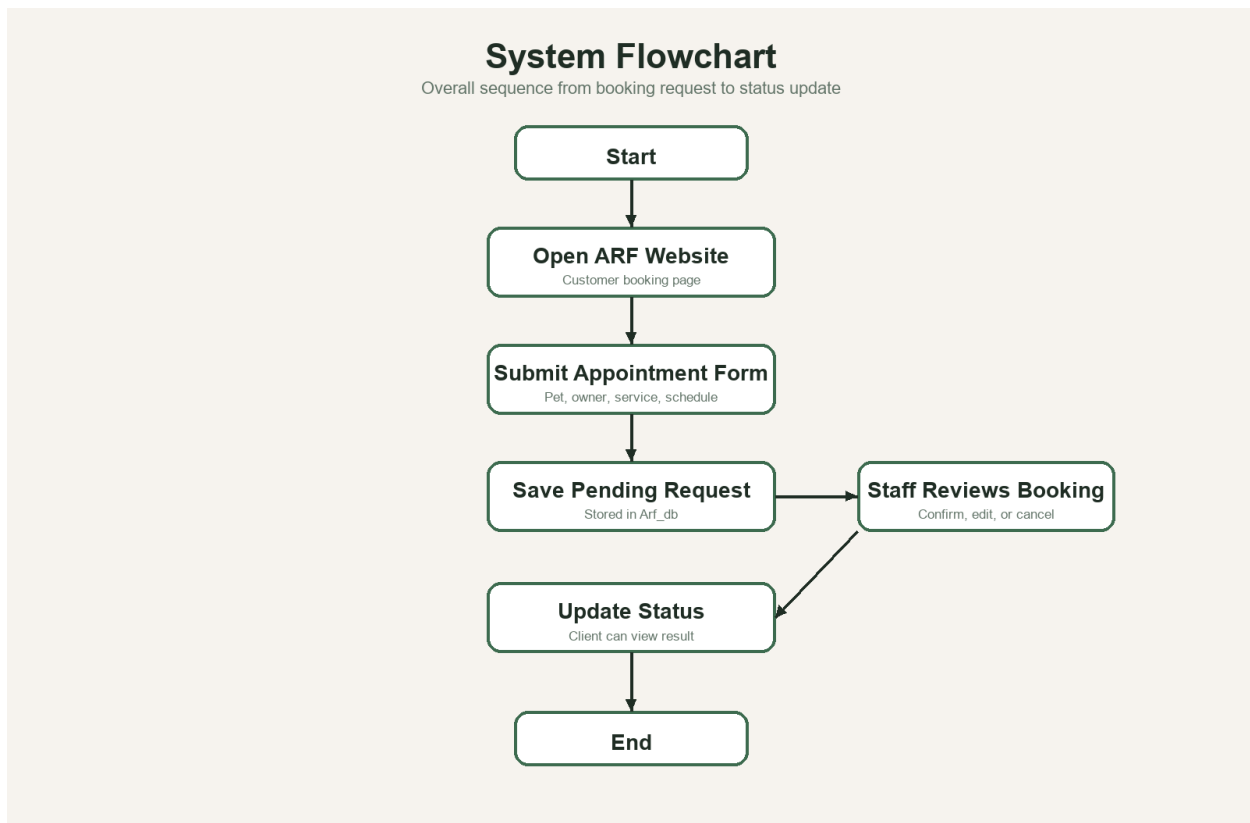
Figure 9. System Flowchart of the ARF Portal
